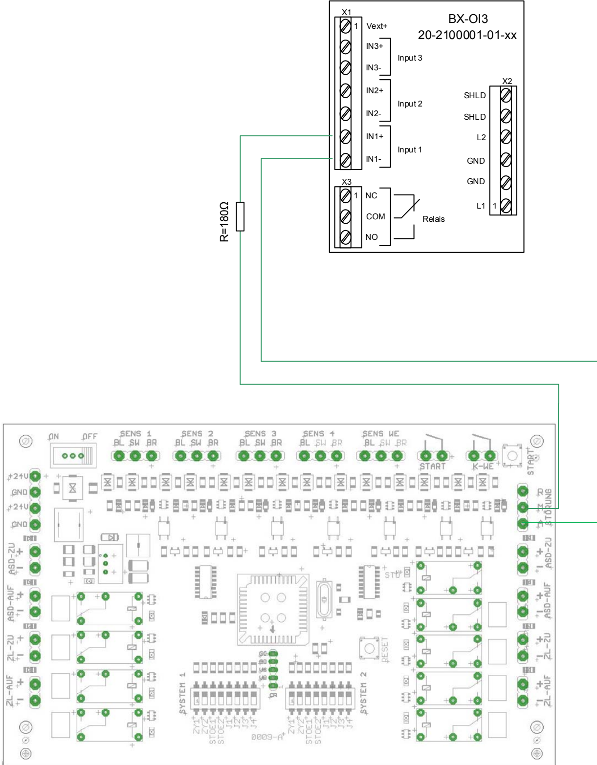
Fig. 9 Activation of fault output with loop module BX-OI3
