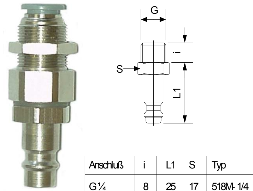
Fig. 8 Coupling plug NG 8 (G 1/4)
