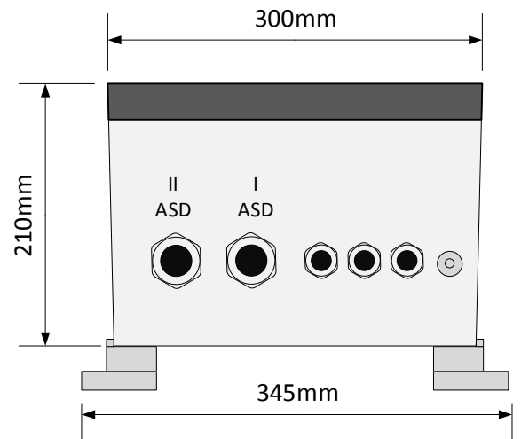
Fig. 5 Drilling plan ADB 2000
