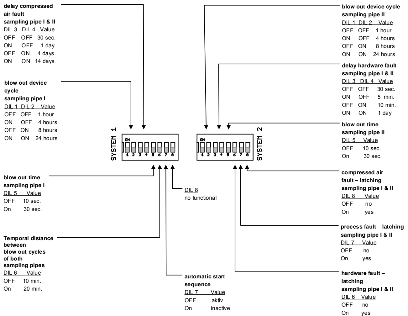
Fig. 10 DIL switch configuration
