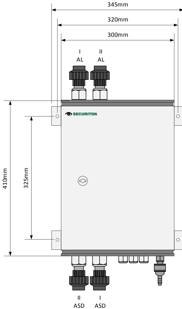
Fig. 4 Drilling plan ADB 2000
