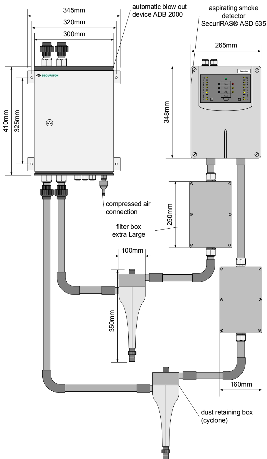
Fig. 6 Standard installation with dust retaining box (cyclone principle) and extra-large filter box
