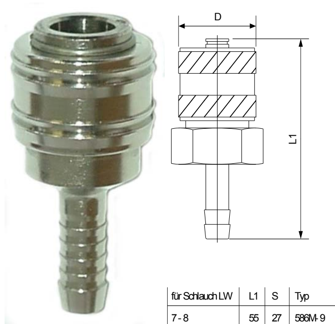
Fig. 7 Coupling socket NG 8 (for 7-8 mm pipe)
