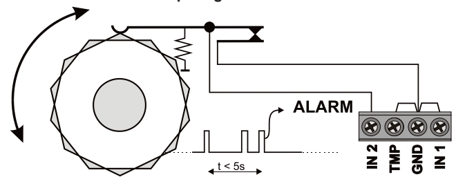
Ratchet-wheel function scheme
