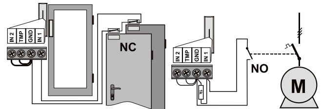
Wiring example for NC ... and NO contacts
